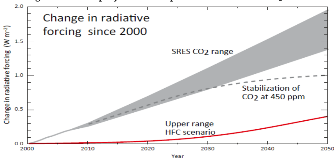
Figure 10. HFCs projected to be up to 20- 40% of RF of CO 2 in 2050
