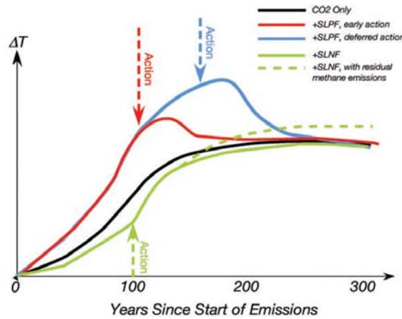
Figure 5. Cooling from SLCP Mitigation in a Carbon Constrained Scenario
