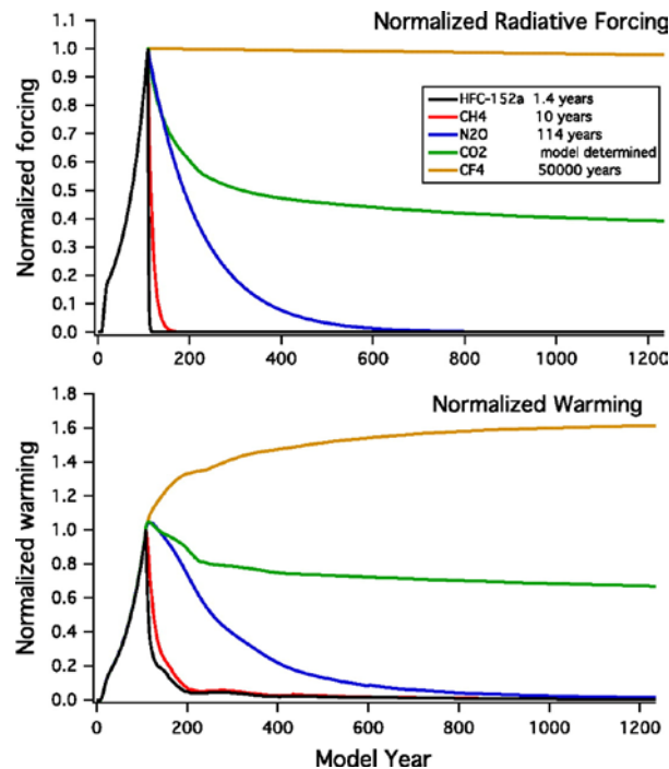
Figure 6. Persistence of Warming From Greenhouse Gases
