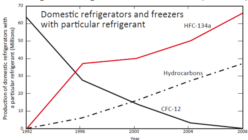
Figure 11. Annual global production of domestic refrigerators and freezers, showing changes in the refrigerants used from 1992 to 2008 (RTOC 2011).
