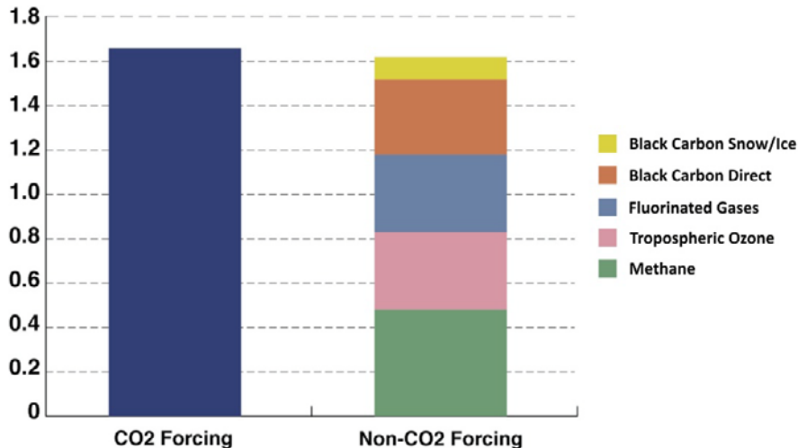
Figure 1. Changes in radiative forcing from anthropogenic emissions since the Industrial Revolution of 1750 (in W/m 2 )
