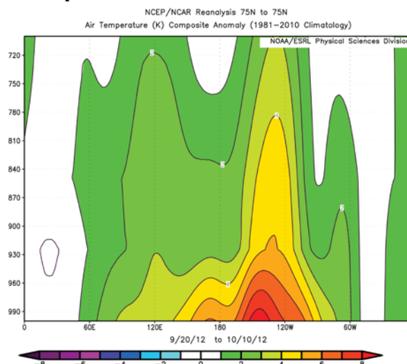
Figure 7. Open Water Warms the Lower Atmosphere
