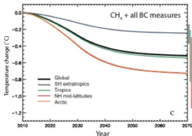
Figure 9. Regional Temperature Benefits From SLCP Mitigation
