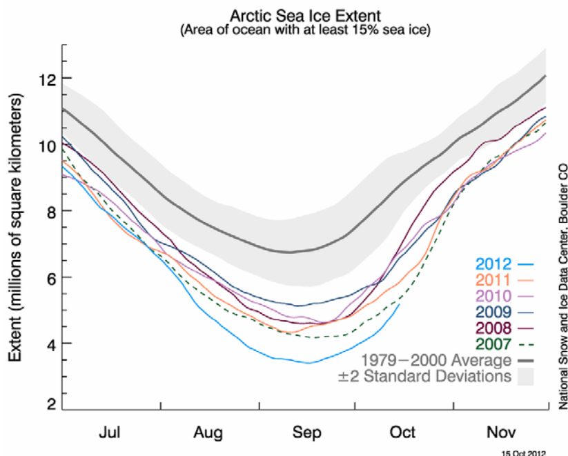
Figure 8. Collapsing Arctic Summer Sea-Ice
