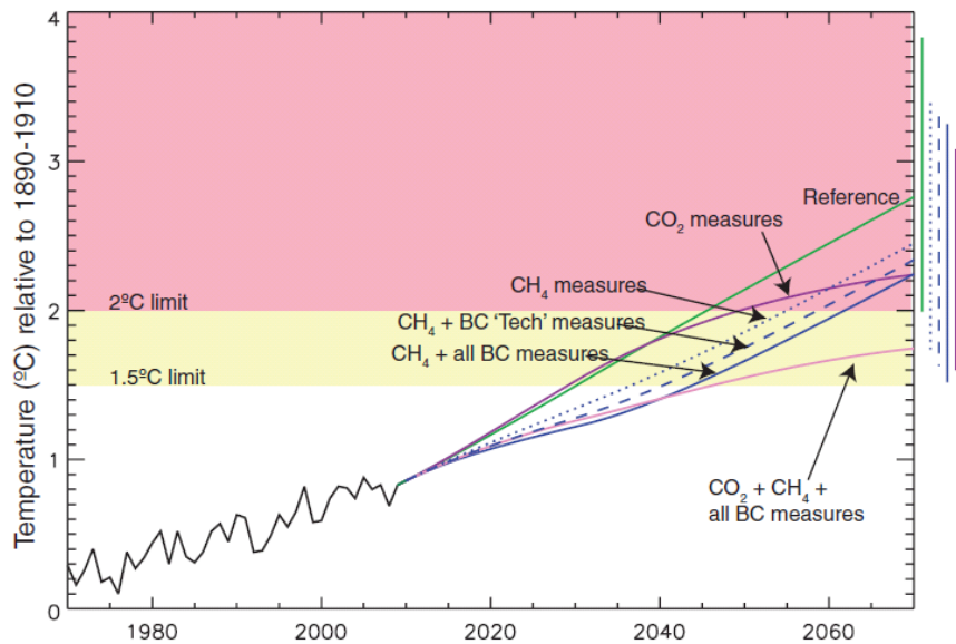
Figure 4. Temperature Rise Predictions Under Various Mitigation Scenarios
