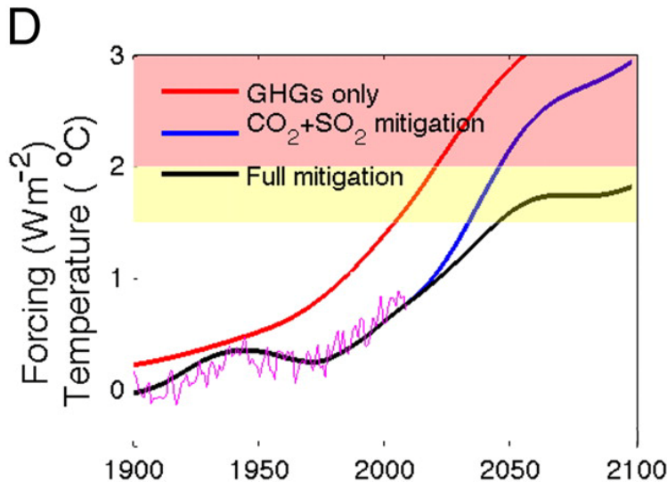
Figure 3. Warming Avoided Through Combined SLCP and CO 2 Mitigation
