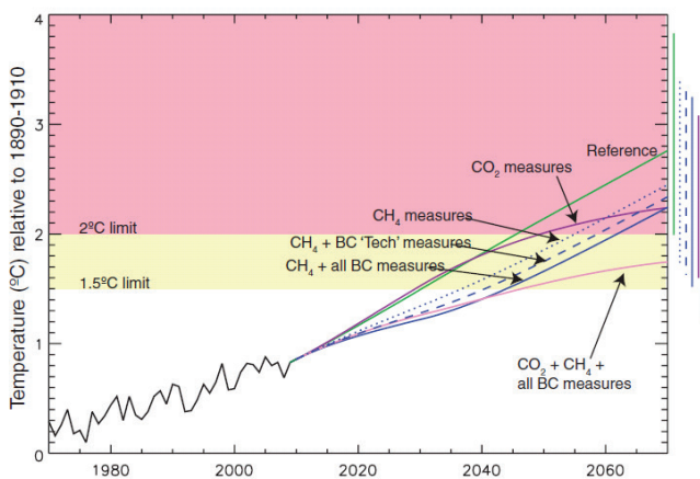
Figure 4. Temperature Rise Predictions Under Various Mitigation Scenarios
