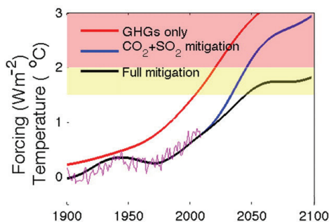
Figure 3. Warming Avoided Through Combined SLCP and CO 2 Mitigation
