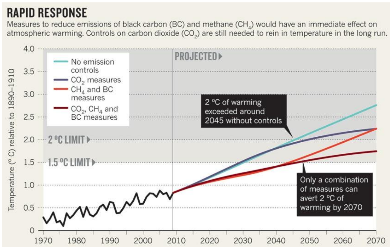
Fig. 3. Temperature Rise Predictions Under Various Mitigation Scenarios
