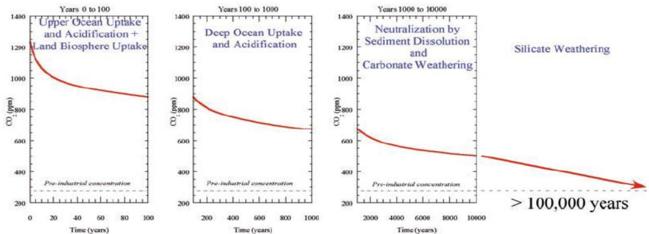
Fig. 2. Time Scales for Removal of CO 2 from the Atmosphere
